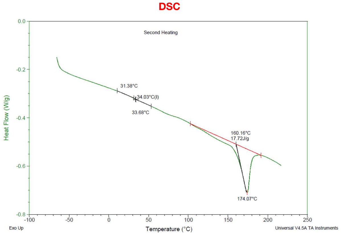
Figure 1. 2nd heating scan DSC data for the Nylon 12 Flat (XY) sample.
